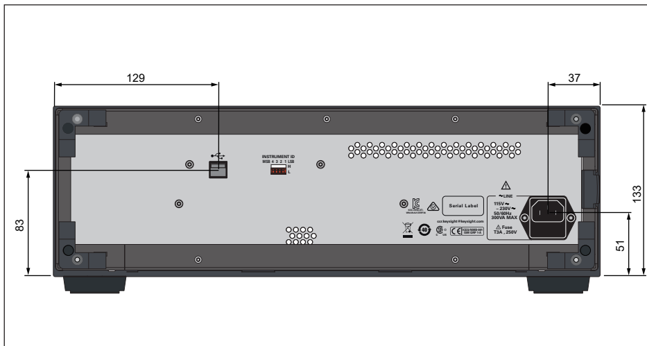
Figure 12. Dimensions (rear view, with Option E5092A-020, in millimeters, nominal)
