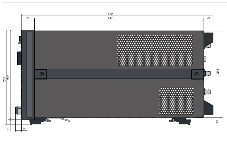
Figure 9. Dimensions (side view, E5071C with Option 2D5/2K5/4D5/4K5, in millimeters)
